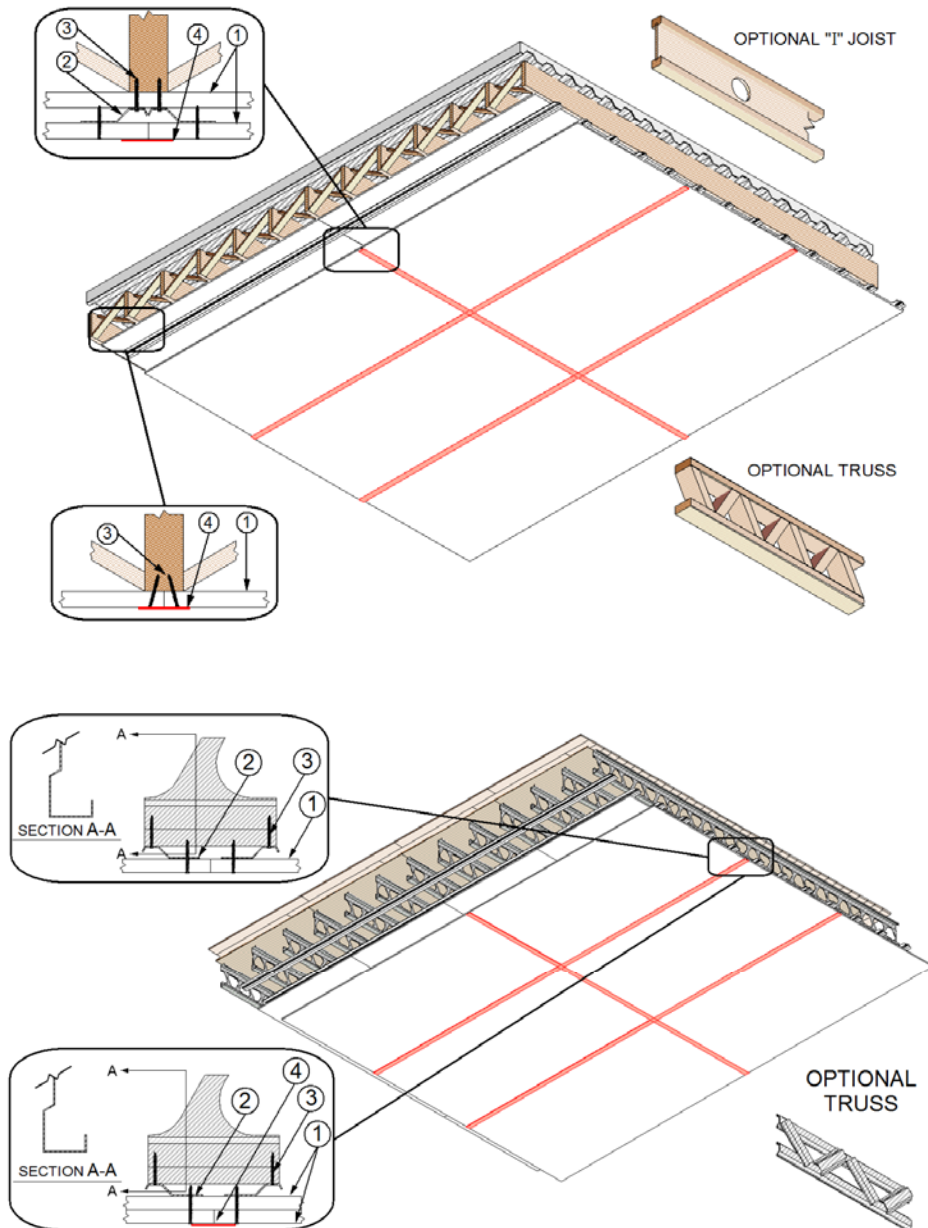
Figure 1 – Floor/Ceiling Assembly & Details
