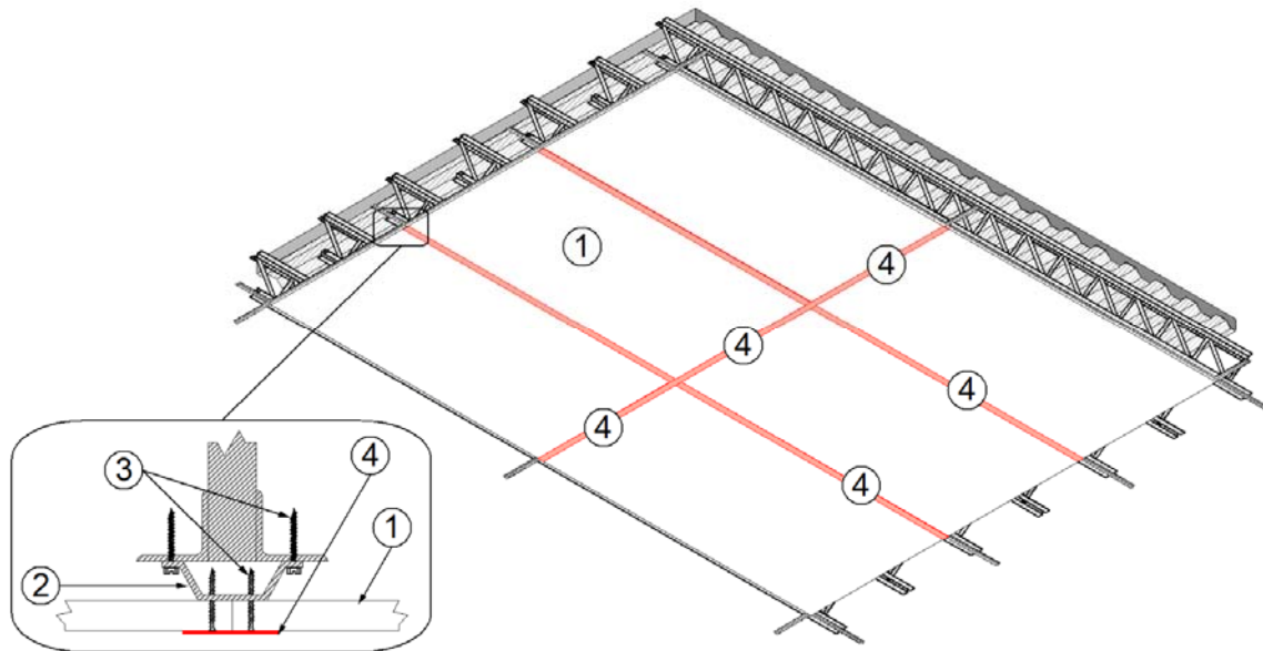
Figure 1 – Floor/Ceiling Assembly & Details
