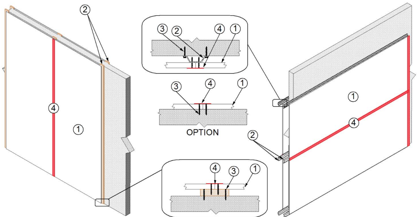
Figure 1 – Wall Assembly & Details
