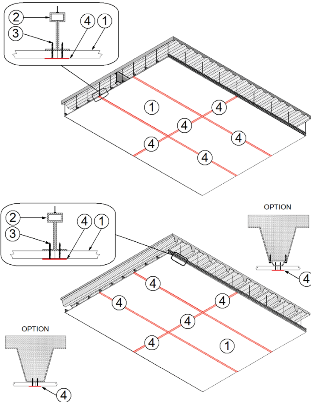
Figure 1 – Floor/Ceiling Assembly & Details
