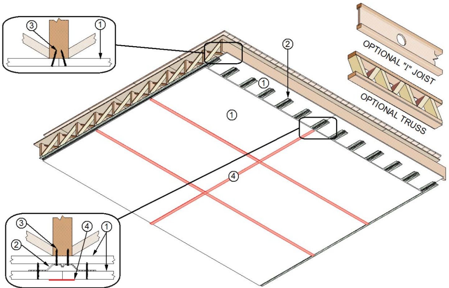
Figure 1 – Floor/Ceiling Assembly & Details
